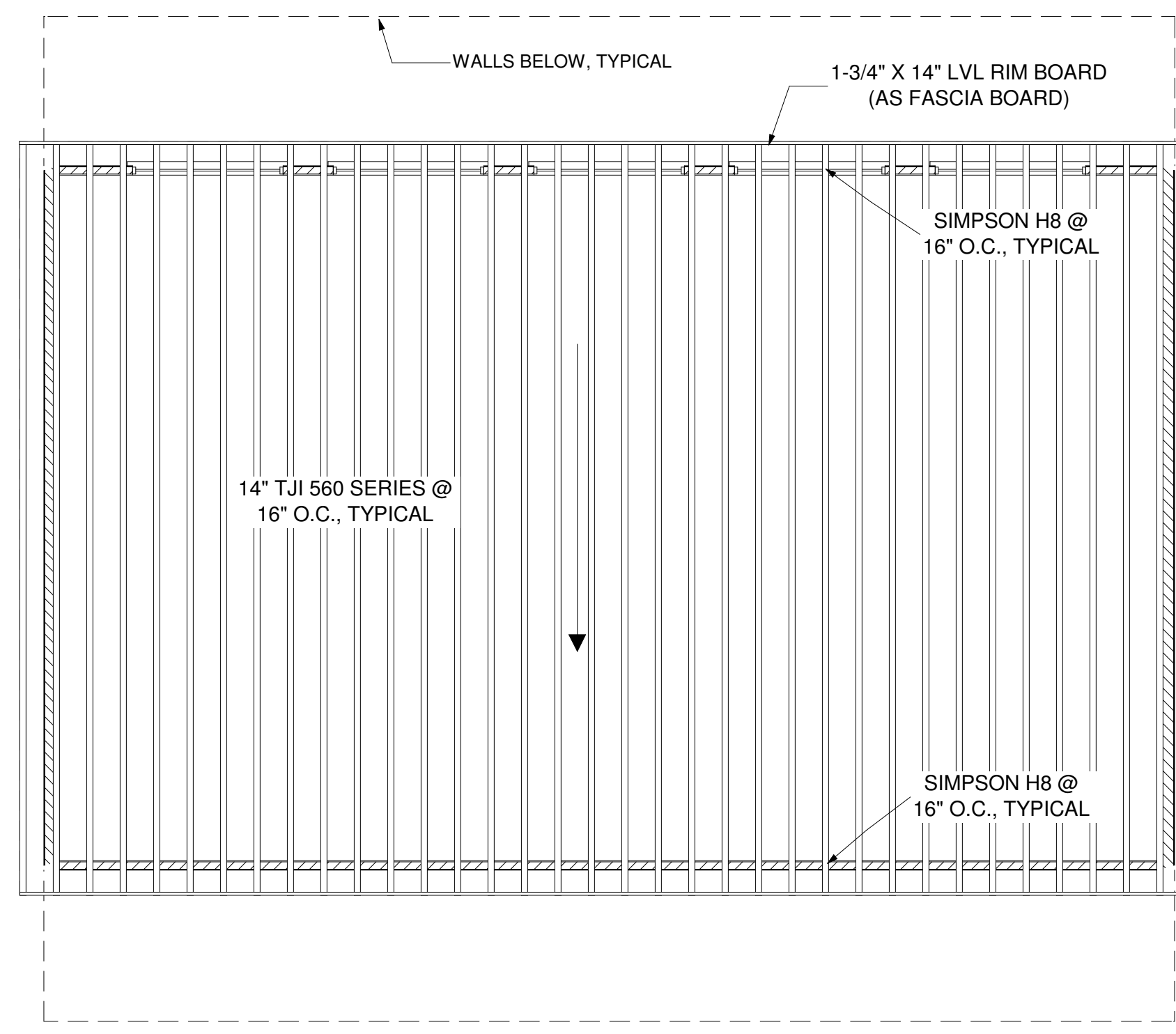
UPPER ROOF PLAN SCALE: 3/16" = 1'-0"
