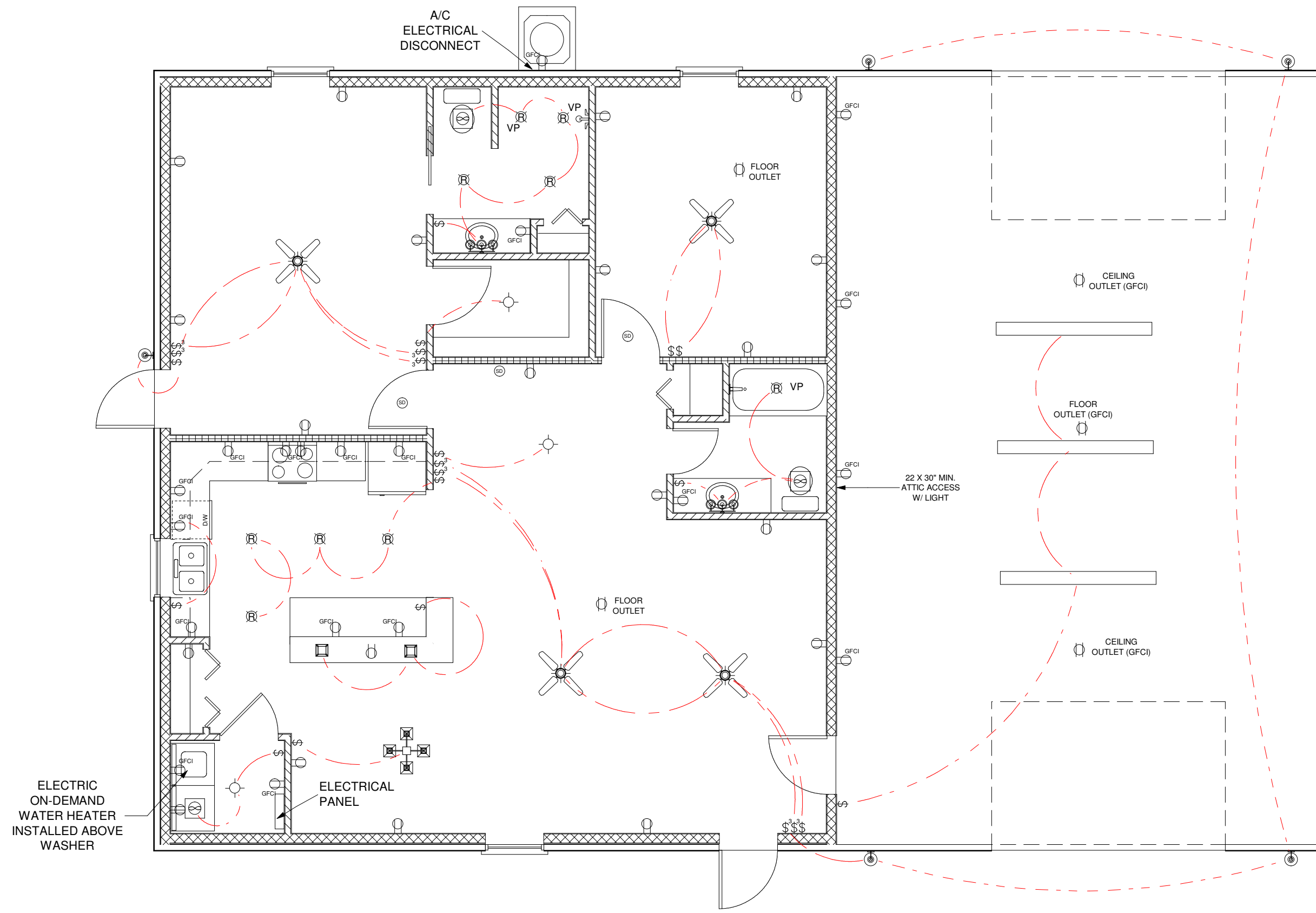
ELECTRICAL PLAN SCALE: 3/16" = 1'-0"
