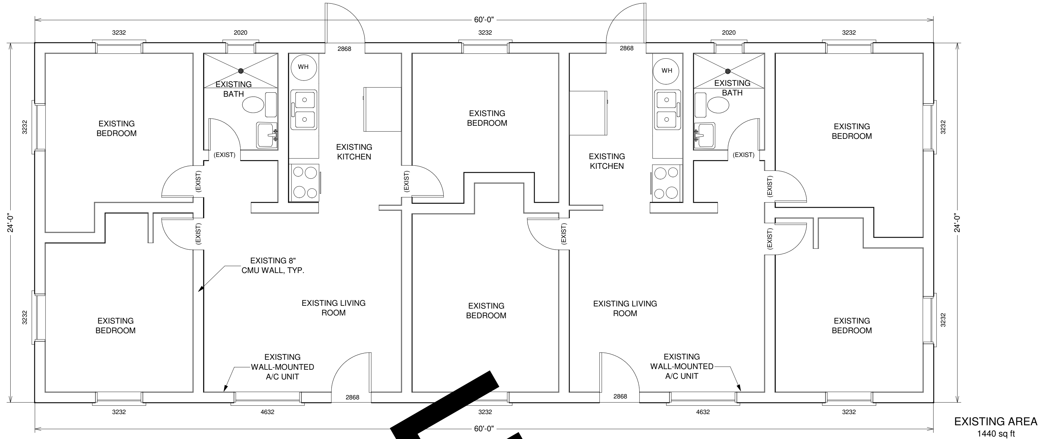
EXISTING FLOOR PLAN SCALE: 1/4" = 1'-0"
