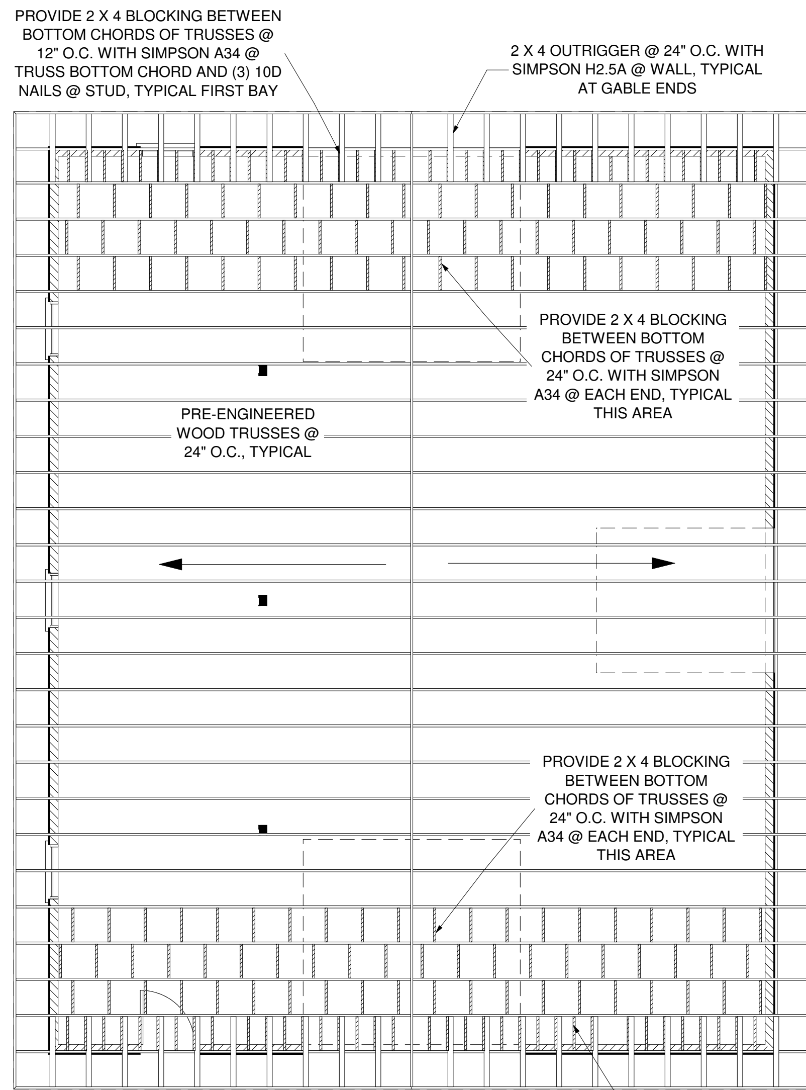
ROOF FRAMING PLAN SCALE: 3/16" = 1'-0"
