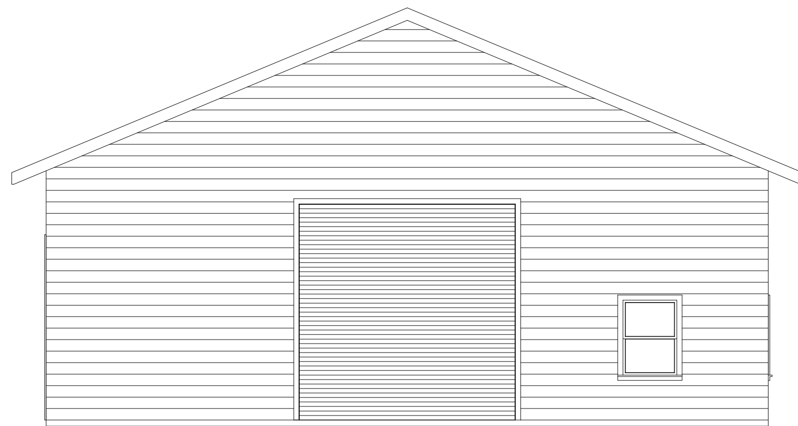
REAR ELEVATION SCALE: 3/16" = 1'-0"
